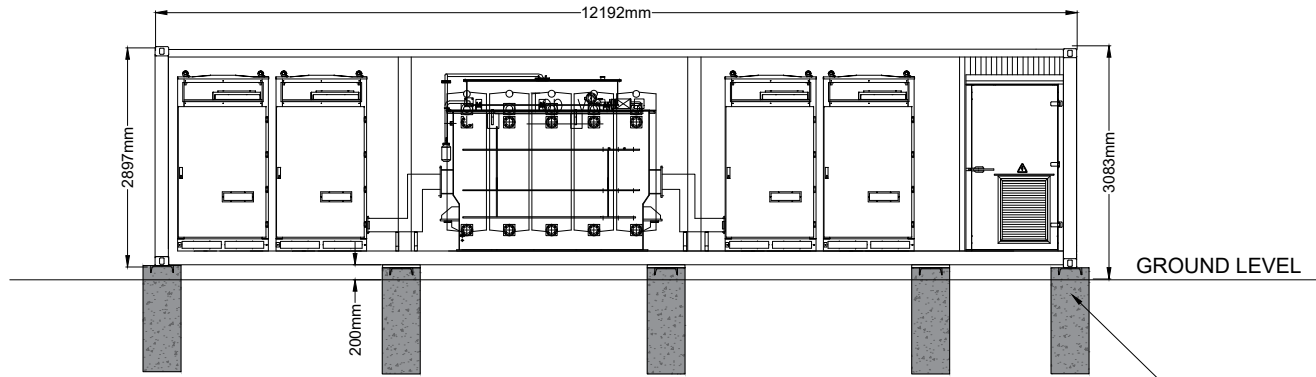
NORTHERN ELEVATION
