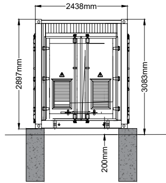
EASTERN ELEVATION
