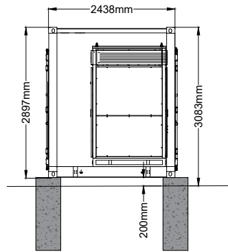
WESTERN ELEVATION
