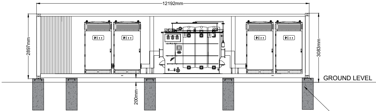
SOUTHERN ELEVATION
